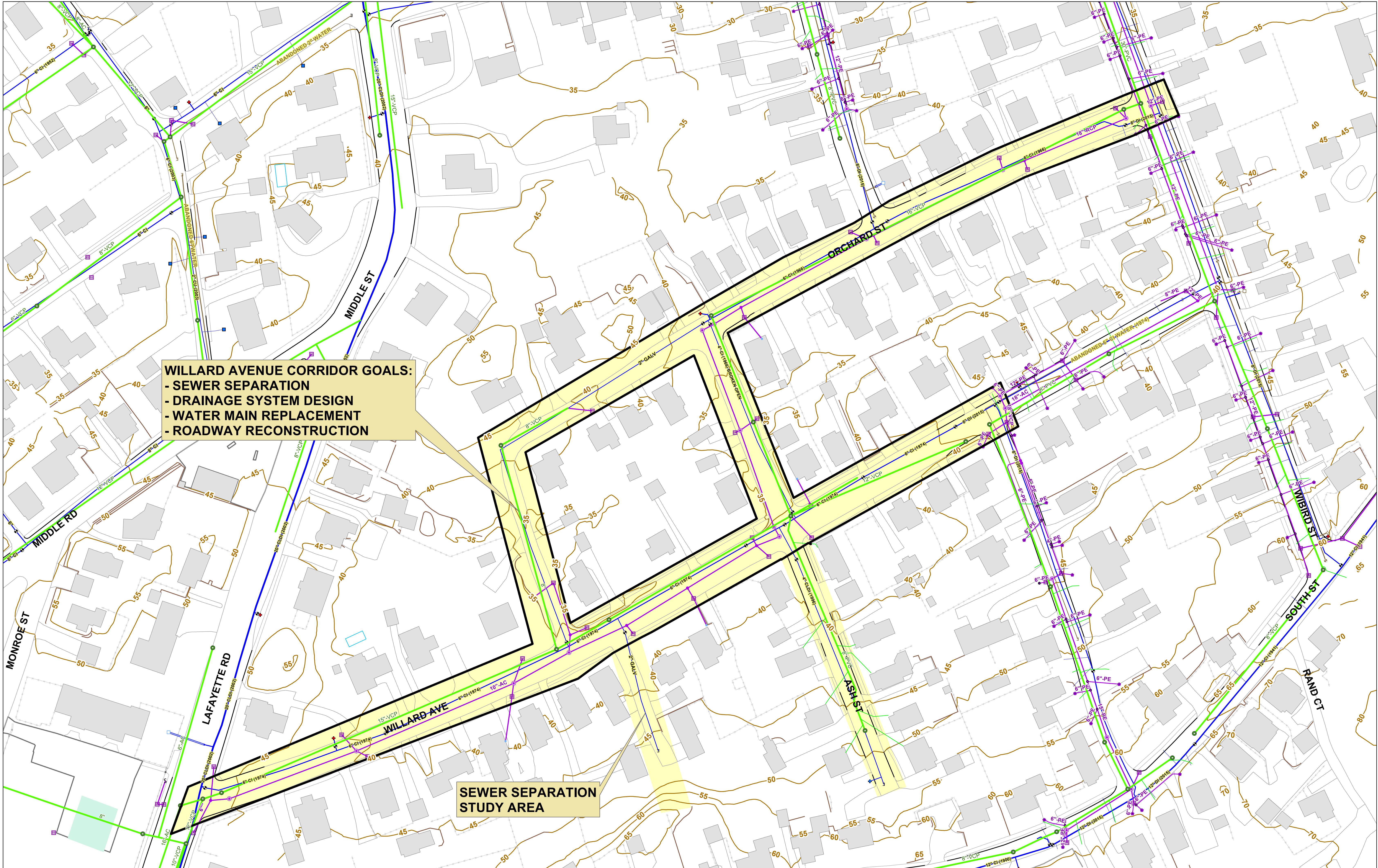
FIGURE 2: WILLARD AVENUE RECONSTRUCTION
